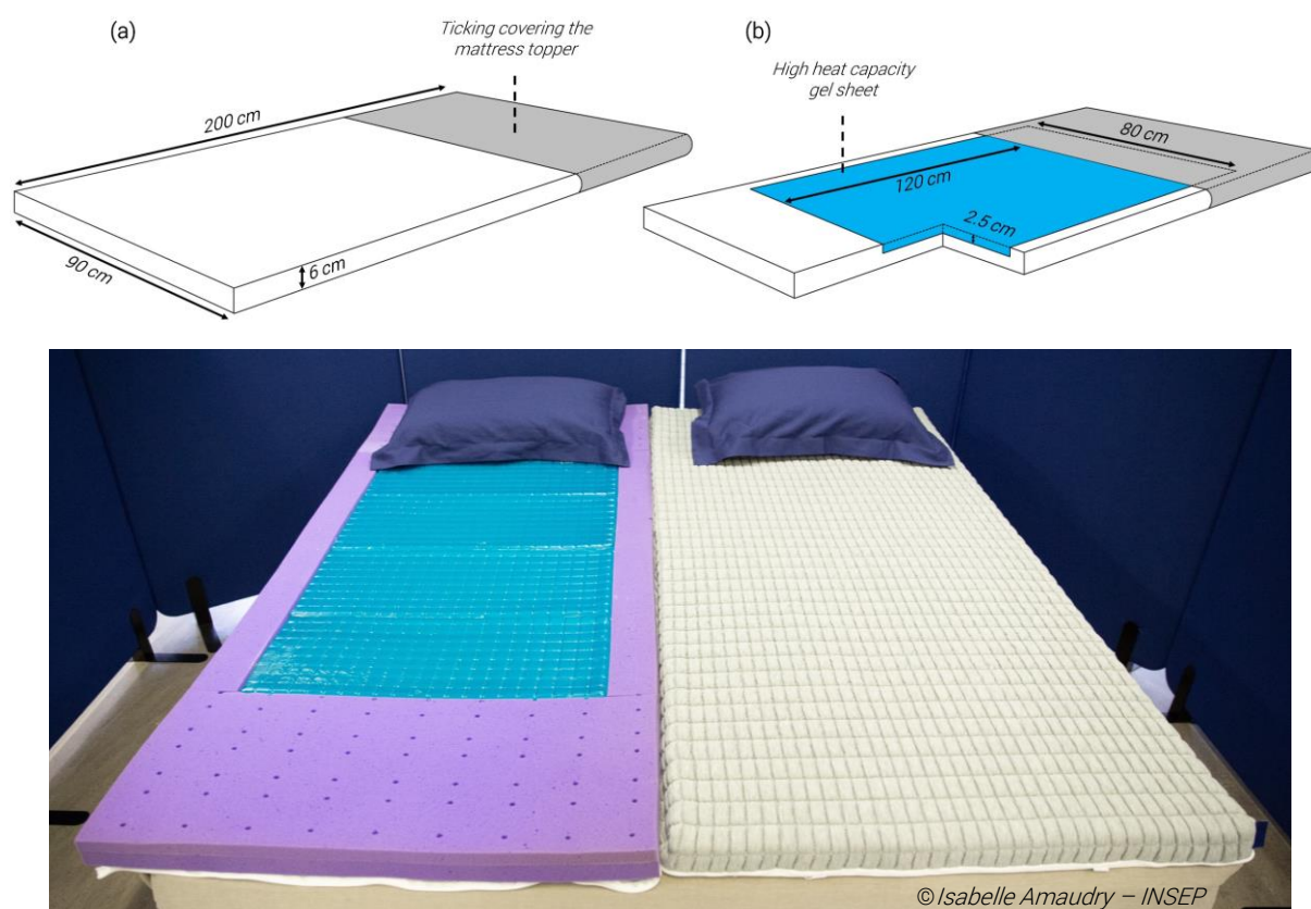
Figure 18. Figure illustrating the design of the low- (a) and high- (b) heat-capacity mattress topper. Picture represents the high-heat-capacity mattress topper without (left) and with (right) the ticking.
