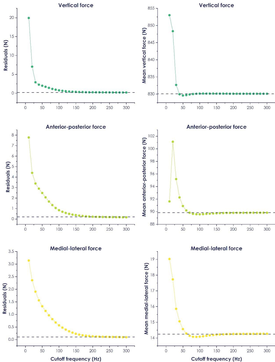
Figure 28. The left panels correspond to the plots of the residuals between the raw vertical, antero-posterior and medial-lateral ground reaction forces (GRF) and the filtered signals over 3 stances as a function of the filter cut-off frequency. For each panel, the horizontal dotted line corresponds approximately to the "stability point". This means that starting from this cut-off frequency, choosing a higher cut-off frequency will result in negligible changes in the residuals. The right panels show the change in the mean vertical, antero-posterior and medial-lateral GRF over 3 stances as a function of the filter cut-off frequency. The horizontal dotted line also corresponds to the "stability point", meaning that an increase in the cut-off frequency will not affect the mean GRF starting from this point.
