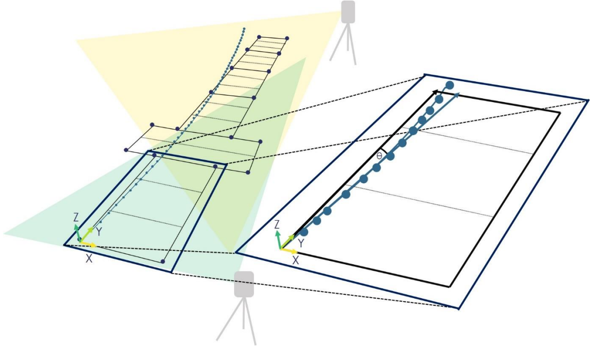
Figure 31. Graphical representation of the angle between the force platforms' (FP) global coordinate system and each zone's vector. The right-hand side of the figure is a zoom in of the first FP. The angle \theta corresponds to the angle between the Y-axis of the FP (black arrow) and the curve (blue arrow). On each panel, the dark dashed lines correspond to the separation of each force platform's areas.
