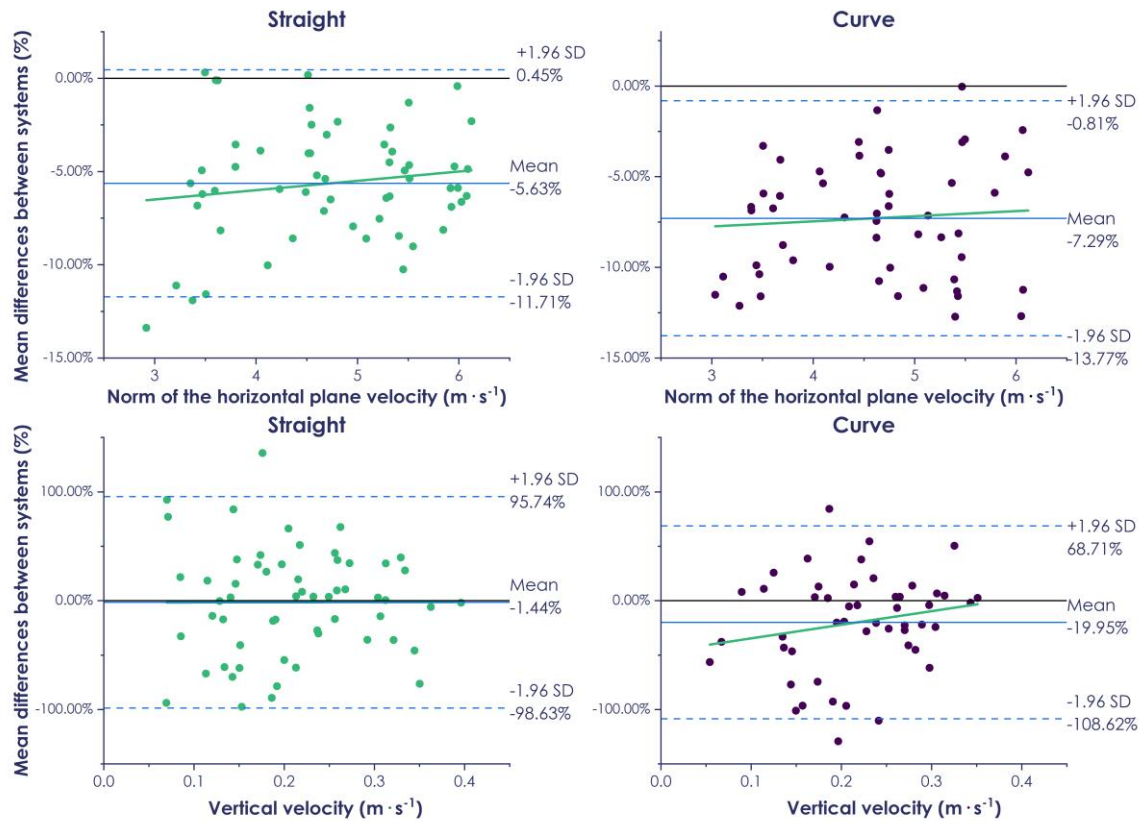
Figure 39. Bland & Altman plots presenting the mean differences (blue horizontal line) and 95% limits of agreement (dashed horizontal lines) between the norm of the horizontal plane velocity computed with the Magneto-Inertial Measurement Units (MIMU)-based system ( V_{H\ MIMU} ) and the force platforms ( V_{H\ FP} ) (panels A & B); between the vertical velocity computed with the MIMU-based system ( V_{V\ MIMU} ) and the force platforms ( V_{V\ FP} ) (panels C & D) for the stances at 0-6 m both in the straight (panels on the left) and the curve (panels on the right). The green line is a linear fit from all individual points.
